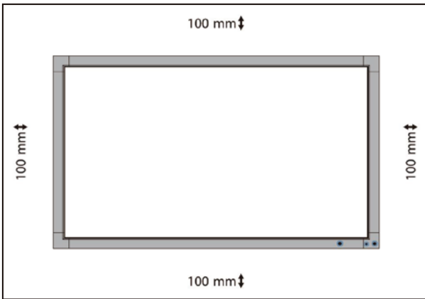
Figure 4 Ventilation Area
